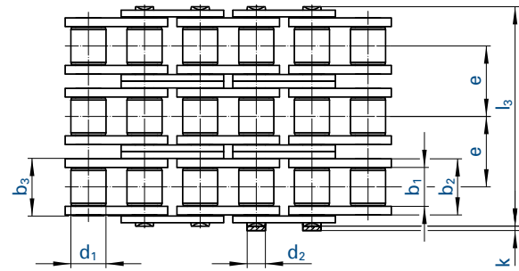
Connecting side
