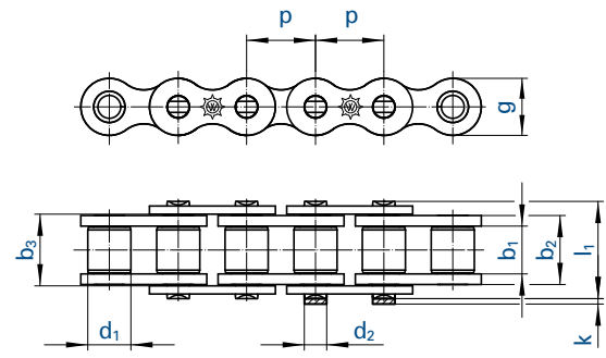
Connecting side
